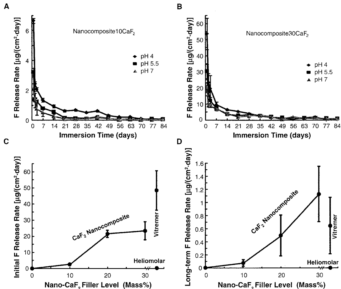
Figure 4. Fluoride release rate, which is the F release per specimen surface area per day (mean \pm SD; n = 3 ). Each error bar shows 1 standard deviation. (A) Nanocomposite10CaF 2 and (B) Nanocomposite30CaF 2 , (C) Initial F-release rates. Vitremer had the highest initial release [ 48.4 \pm 12.3 \mu\text{g}/(\text{cm}^2\cdot\text{day}) ], followed by 23.4 \pm 5.6 for Nanocomposite30CaF 2 , 21.5 \pm 2.2 for Nanocomposite20CaF 2 , 2.4 \pm 0.2 for Nanocomposite10CaF 2 , and 0.17 \pm 0.04 for Heliomolar ( p < 0.05 ). (D) Long-term F-release rates were 1.13 \pm 0.42 for Nanocomposite30CaF 2 , 0.65 \pm 0.43 for Vitremer, and 0.50 \pm 0.31 for Nanocomposite20CaF 2 ( p > 0.1 ). They were higher than 0.10 \pm 0.05 of Nanocomposite10CaF 2 and 0.006 \pm 0.003 of Heliomolar ( p < 0.05 ).
